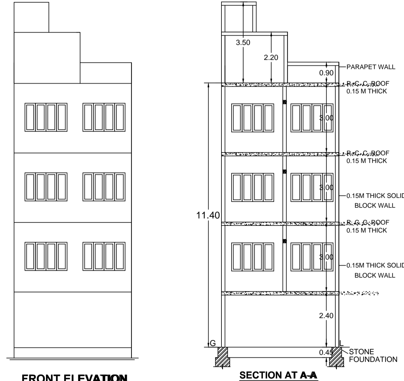
FRONT ELEVATION
